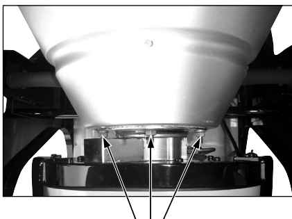
Unscrew three nuts and take the burner unit off
